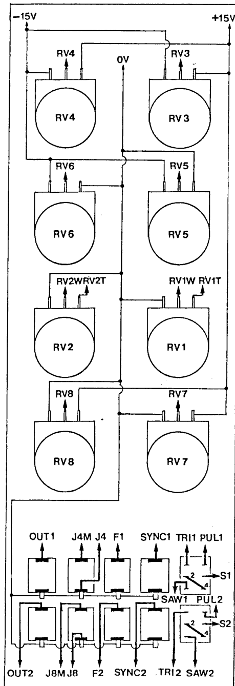
FIGURE 4. 80-19 PANEL WIRING
